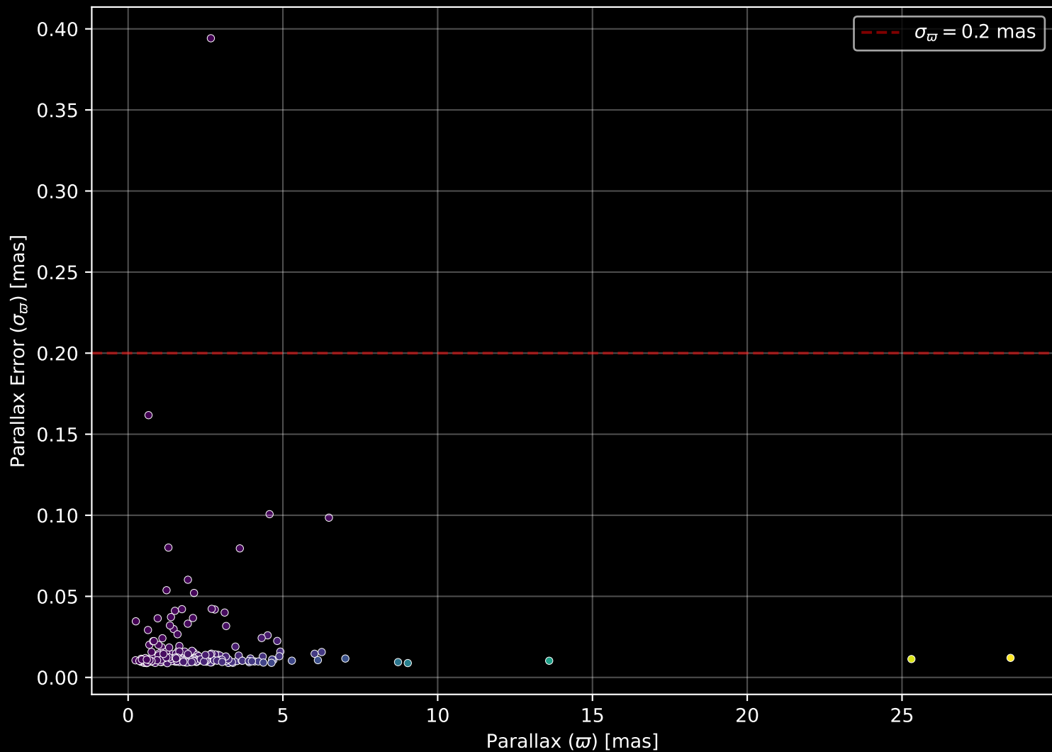
GALAH DR4 Field: [7225] Parallax Quality (n= 242)
