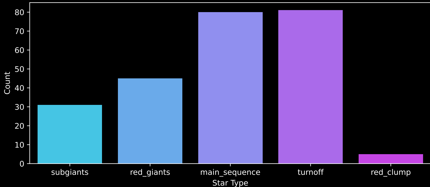
GALAH DR4 Field: [7225] Count plot of Star Type
