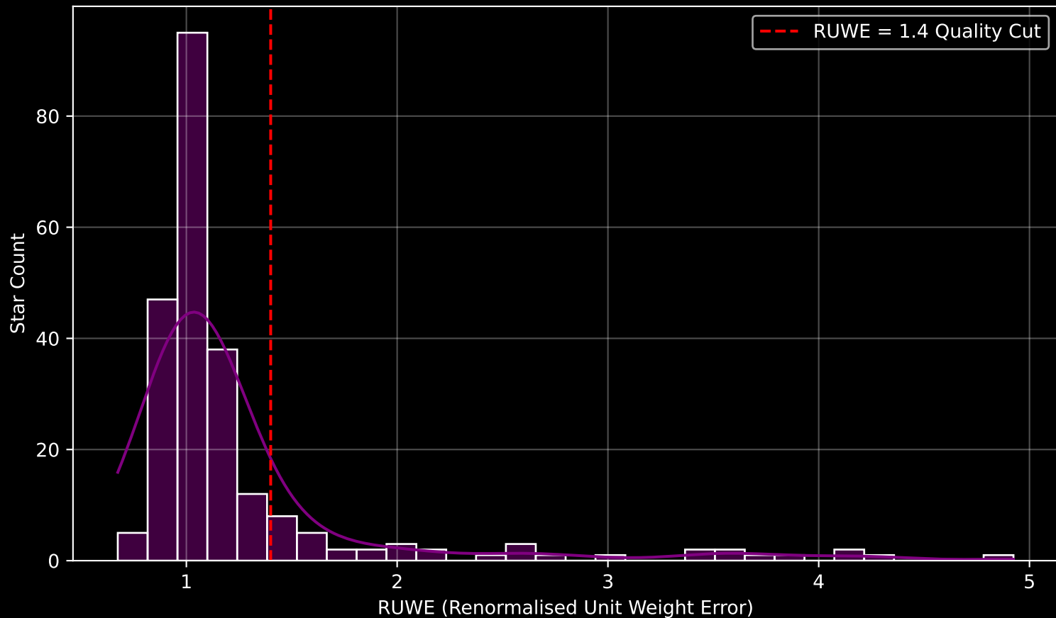
GALAH DR4 Field [7225] RUWE Distribution (n= 235)
