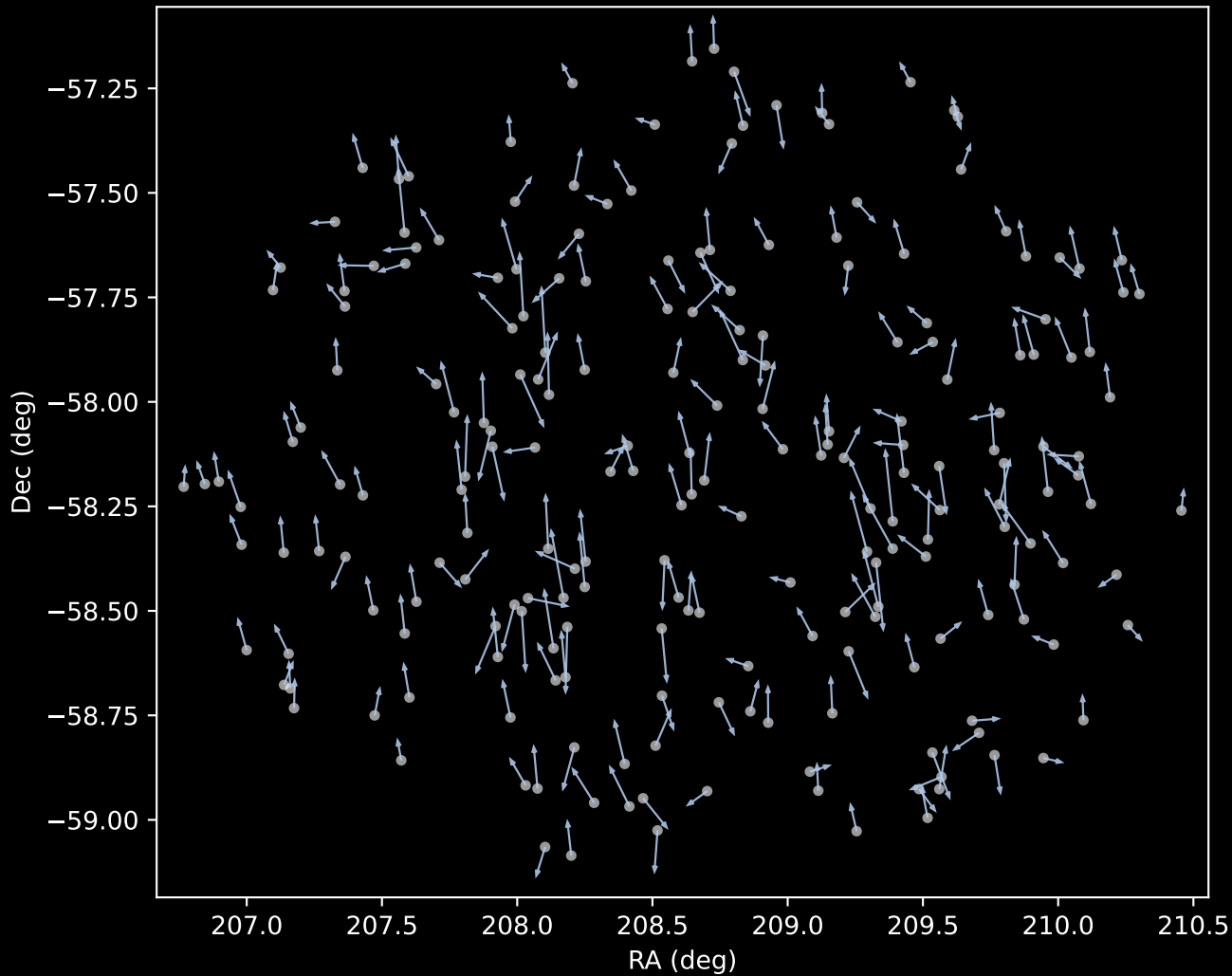
GALAH DR4 Cluster 1 Proper Motion Vectors (n=217)
