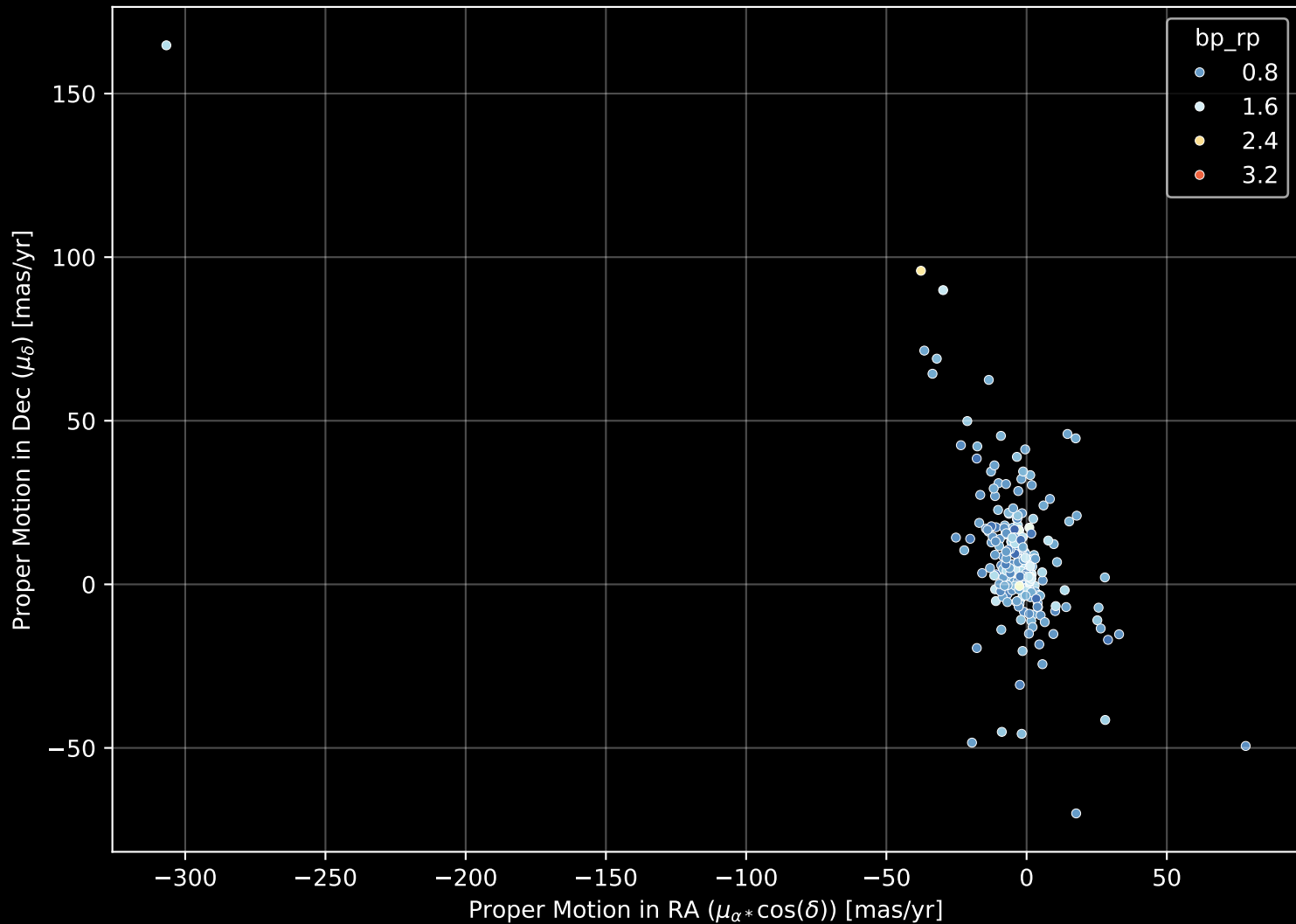
GALAH DR4 Field: [7225] Proper Motion Diagram (n= 242)
